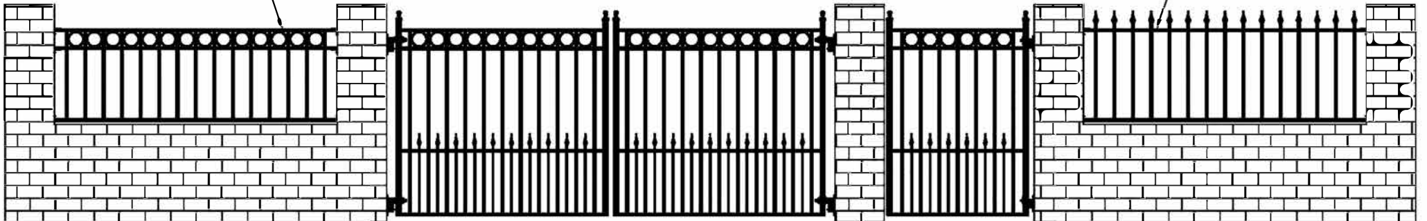
OPTION #1: MONTEREY FENCE PANEL 2300mm(7' 6") GAP WIDTH x 755mm(2'6") HIGH
